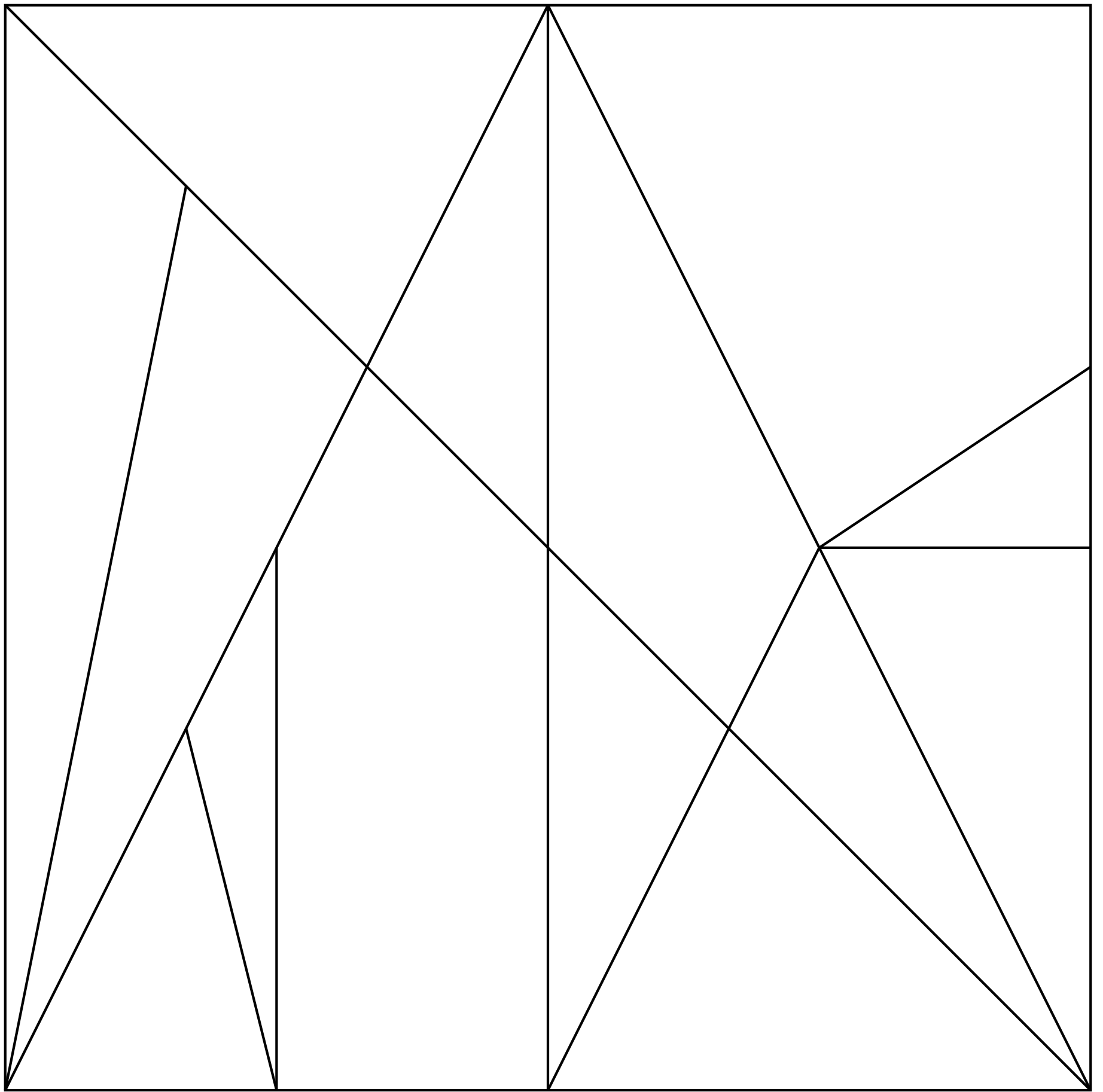
Ostomachion (after Suter)
